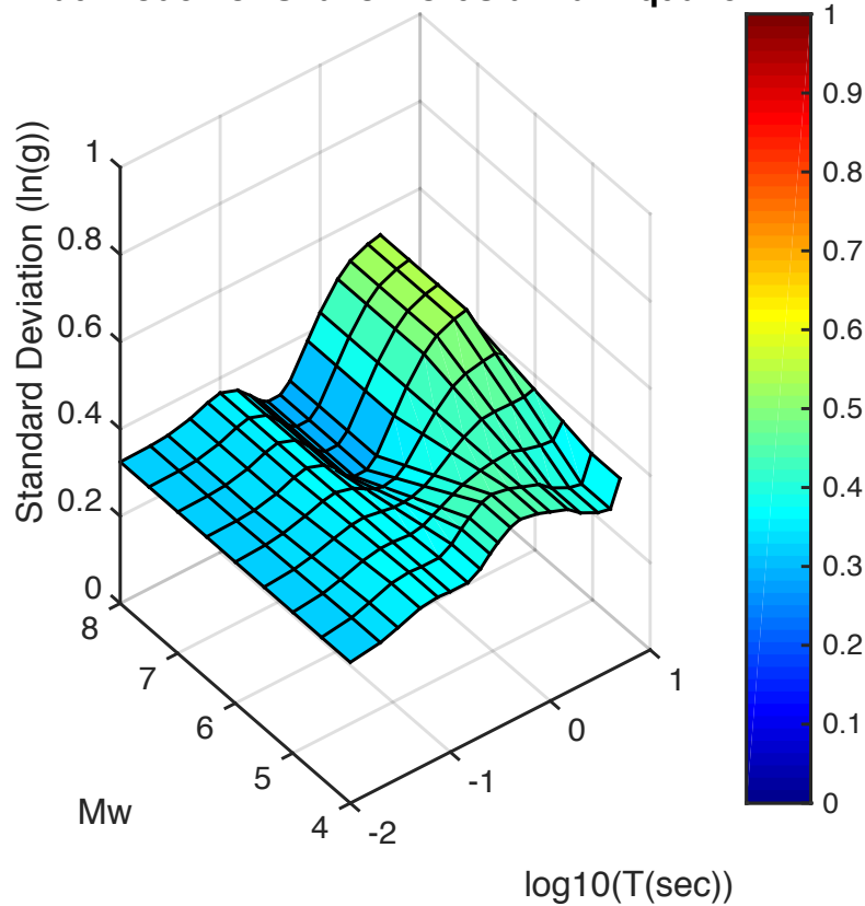
Tau Model for Shallow Crustal Earthquake
