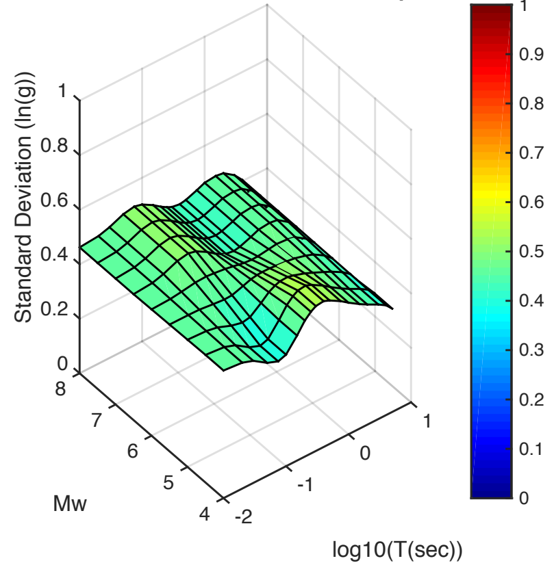
Phiss Model for Subduction Earthquake
