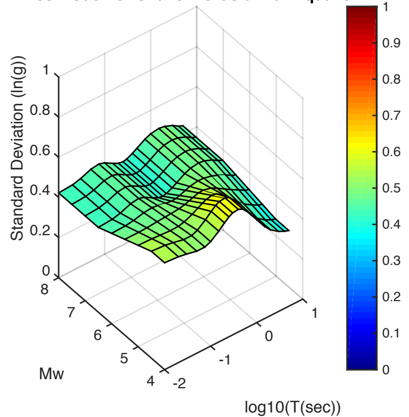
Phiss Model for Shallow Crustal Earthquake
