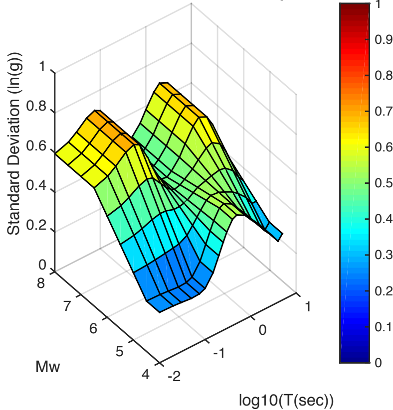
Tau Model for Subduction Earthquake
